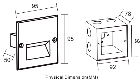
Physical Dimension(MM)
