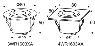
Physical Dimension(MM)
