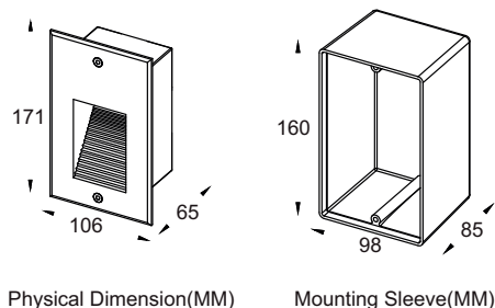
Physical Dimension(MM)
