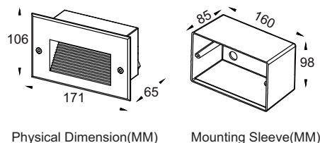
Physical Dimension(MM)
