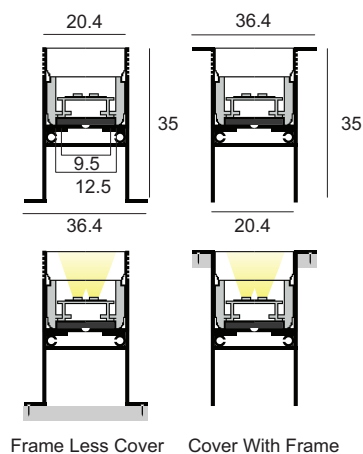
Frame Less Cover Cover With Frame
